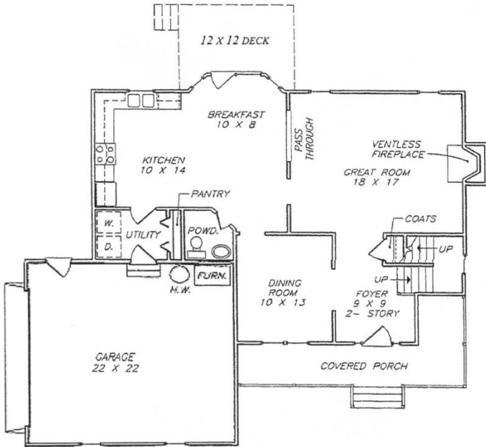
First Floor 9 ft. Ceilings
